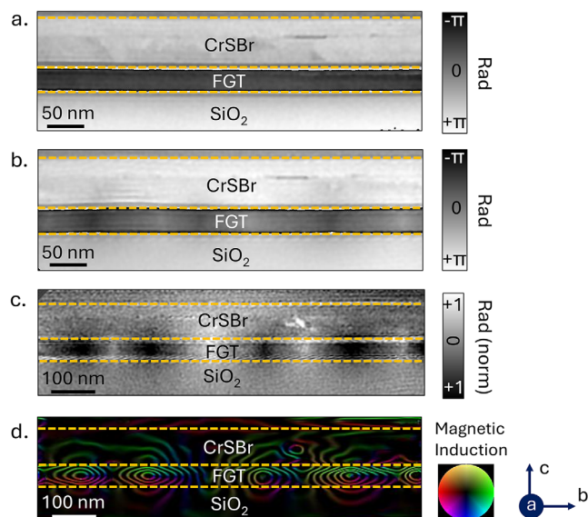
Figure 3. Electron Holography images of the CrSBr/FGT heterostructure along the bc plane measured at 0 mT field and 95 K. a) Phase map measured at zero field after application of a 1 T field along the c axis. b) Phase map of the demagnetized state. c) Magnetic phase image of the zero-field cooled state after subtraction of the nonmagnetic contribution using a phase image acquired above the T_C of FGT. d) Color-coded phase gradient map that shows the direction of the magnetic induction field B with a contour spacing of 2\pi/30 .
