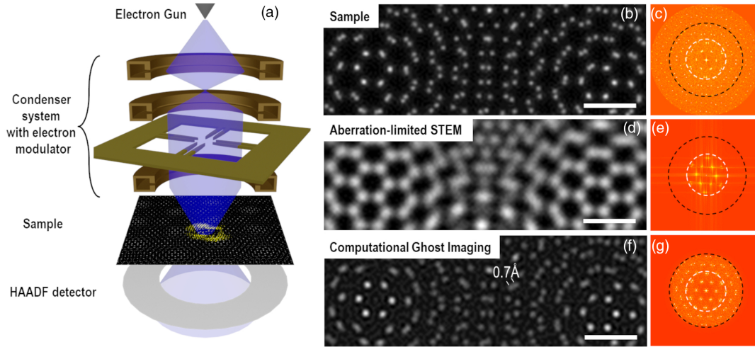
FIG. 1. (a) Schematic representation of the electron-optical setup. (b),(d),(f) Comparison between an MoS 2 twisted bilayer atomic potential, an aberration-limited STEM image, a CGI reconstruction, and (c),(e),(g) their FFTs, in which the light circle corresponds to a semiconvergence angle of 2\alpha , while the dark circle corresponds to 4\alpha . The scale bars are 5 Å.
