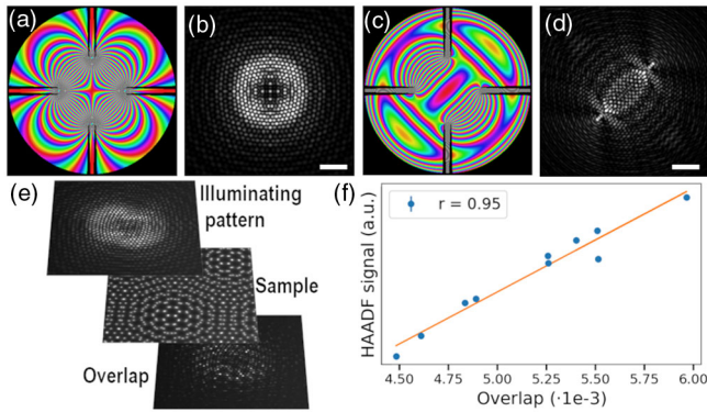
FIG. 2. (a) Phase profile produced by the electron modulator in a centrosymmetric condition without the effect of Cs and (c) with Cs = 2.7 mm, and (b),(d) the corresponding probe shapes; (e) similarity between the patterns and the sample crystal structure, maximizing the overlap. (f) ADF signal computed using a multislice simulation plotted as a function of the overlap of the probe with a 19.2-nm-thick Si [110] sample. The legend gives the Pearson correlation coefficient ( r ).
