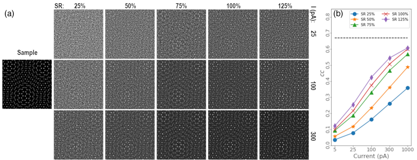
FIG. 3. Effect of sampling ratio on reconstructed image quality for three electron currents. In (a), the same region of a 3.6 \text{ nm} \times 3.6 \text{ nm} simulated sample is reconstructed. (b) shows the behavior of cc as a function of beam current for different SRs. The black dashed line shows the maximum value of cc obtained in the limit of infinite current.
