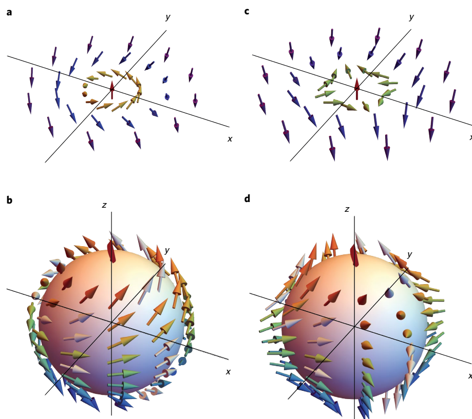
Fig. 1 | Examples of topological magnetic textures. a , A skyrmion with positive topological charge. c , An antiskyrmion with negative topological charge. b,d , The moments wrap around a unit sphere upon application of stereographic projection.
