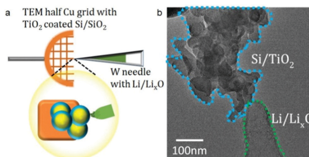
Fig. 2 (a) Schematics of transmission electron microscopy (TEM) half copper grid with titanium oxide (TiO 2 ) coated silicon/silicon oxide (Si/SiO 2 ) nanoparticles and tungsten needle scratched against Li metal, which contains a Li/Li x O fragment as a solid-state electrolyte. (b) Bright-field TEM image showing the open cell configuration used to perform lithiation/delithiation of Si/SiO 2 nanoparticles coated with TiO 2 .
