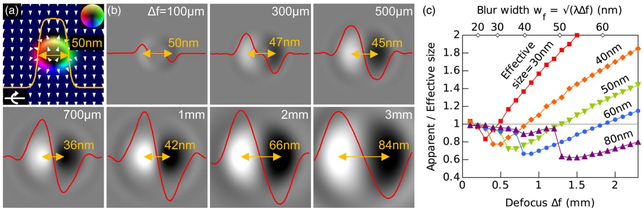
Fig. 5. (a) Theoretical magnetization distribution of a 50 nm Néel-type magnetic skyrmion for a sample tilt angle of 20^\circ (with the tilt axis horizontal). The direction of the magnetization projected in the image plane is given by the colour wheel in the upper right corner and by the white arrows. The yellow curve corresponds to the out-of-plane component of the magnetization projected in the image plane in the horizontal radial direction. (b) Simulated Fresnel defocus images calculated from the model shown in (a) for the different defocus values indicated in the images. The red curves correspond to intensity profiles in the horizontal radial direction. The apparent size, i.e., the distance between the peak and the dip, is indicated on each image. (c) The ratio between the apparent size and the effective size of the magnetic skyrmion plotted as a function of defocus for magnetic skyrmions of different effective size. The upper x axis indicates the width of the first Fresnel fringe w_f \approx \sqrt{(\lambda\Delta f)} .
